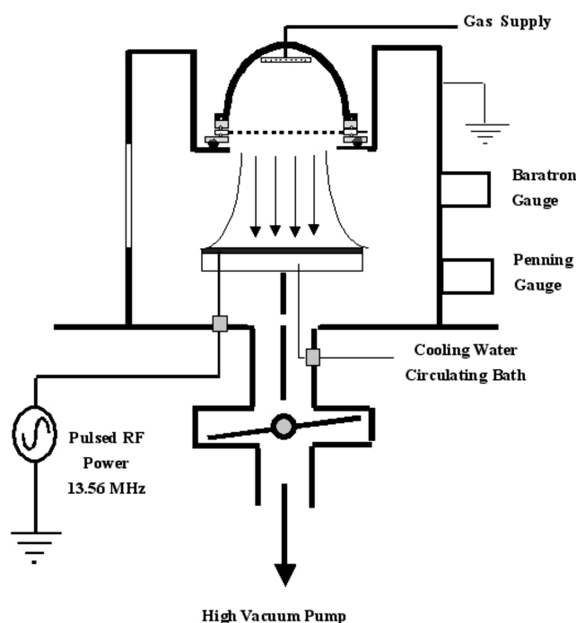
Fig. 1. Schematic diagram of plasma-enhanced chemical vapor deposition apparatus.
